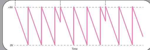
VCO A Sawtooth Wave Output (Sync Engaged)
