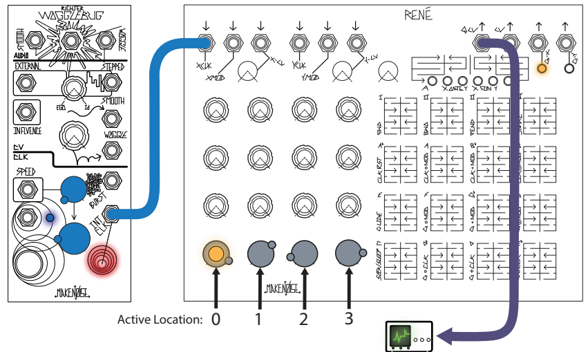
Figure 14: Sequential Voltage
